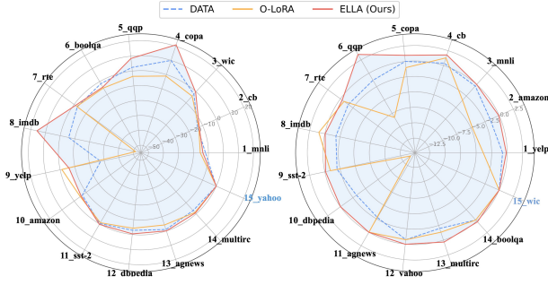
Figure 2: Backward Transfer (BWT) performance for T5-Large model on Long Sequence Benchmark (LS) dataset with Order 4 (left panel) and Order 6 (right panel). ELLA demonstrates superior resistance to performance decline than baselines (higher values indicate better retention of prior task performance).
