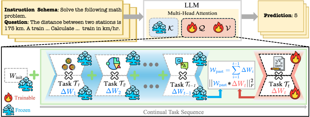
Figure 1: ELLA mitigates interference in continual LoRA training by accumulating past low-rank updates \mathcal{W}_{\text{past}} and applying an energy-based alignment penalty \|\Delta W_t * \mathcal{W}_{\text{past}}\|_F^2 to discourage overlap in high-magnitude, task-specific directions. This selective regularization enables parameter reuse in less-used subspaces, achieving a better trade-off between plasticity and stability without requiring task labels, data replay, or architectural modifications.
