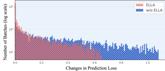
Figure 4: Histogram of prediction loss changes after training on a new task on the T5-Large model. The ELLA constraint helps reduce the changes – preserve the loss of previous tasks – in comparison to when it is not present ( \lambda = 0 ).
