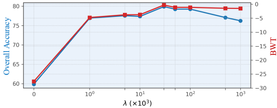
Figure 6: Impact of \lambda scaling on Order 1 of the Standard CL benchmark using the T5-Large model. Overall Accuracy and BWT as \lambda varies shows that moderate scaling achieves the best stability-plasticity balance.
