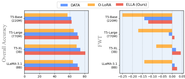
Figure 3: Comparison of Overall Accuracy (OA) and Forward Transfer (FWT) for four models across different backbone size and model families on the Long Sequence Benchmark (LS).
