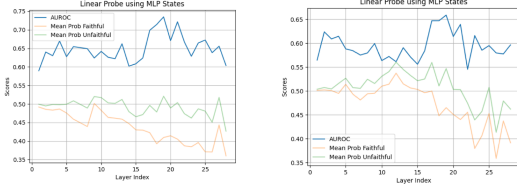
Figure 6: Temporal context drift in hallucination over long reasoning chains. Trained faithfulness detectors may successfully capture the distinction between faithful and unfaithful perception steps early in a model’s generation, they fail as the number of steps in the reasoning trace increases. We train a linear probe detector on the embeddings of each layer, on a dataset with short reasoning traces (left) and test it on longer reasoning traces (right). We report the AUROC (y-axis) for each layer’s linear probe (x-axis). The AUROC drops by around 10 points when evaluated on longer reasoning traces.
