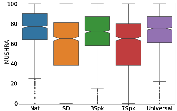
Fig. 4. MUSHRA evaluation for the audiobook data.
