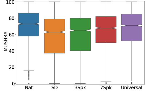
Fig. 3. MUSHRA evaluation for the English, neutral, out-of-domain speakers.
