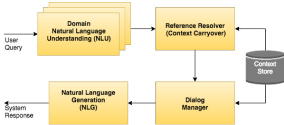
Figure 1: Spoken Dialogue Architecture: A pipelined approach for spoken language understanding. The context carryover system is responsible for resolving references in a conversation and is an input to the dialogue manager.
