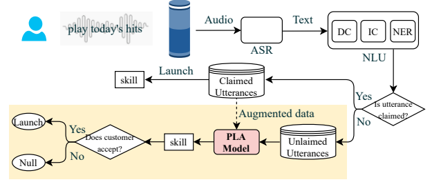
Figure 1: The use case of PLA model in SLU systems.
