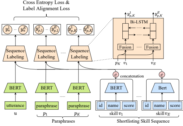
Figure 2: Reranker model \mathcal{R} with Paraphrase label alignment.
