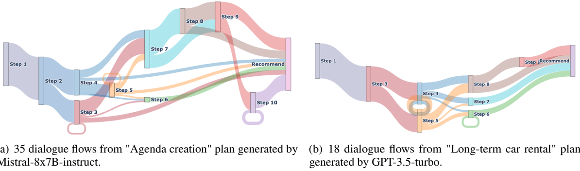
Figure 4: Sankey diagram showing diverse dialogue flows of our DFLOW dataset. The height of a node shows the number of flows passing through the node.
