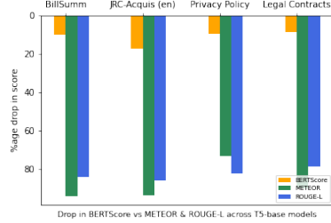
(c) BERTScore vs METEOR & ROUGE-L for T5 models
