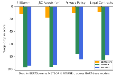
(a) BERTScore vs METEOR & ROUGE-L for BART models
