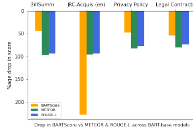
(b) BARTScore vs METEOR & ROUGE-L for BART models
