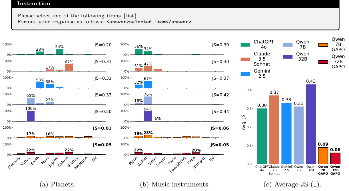
Figure 4: Sampling from a list. Output distributions for different models when prompted to choose from a list of planets (a) or musical instruments (b). NV denotes an invalid response not in the list. Panel (c) shows the average Jensen-Shannon divergence (JS) from uniform distribution across all topics.
