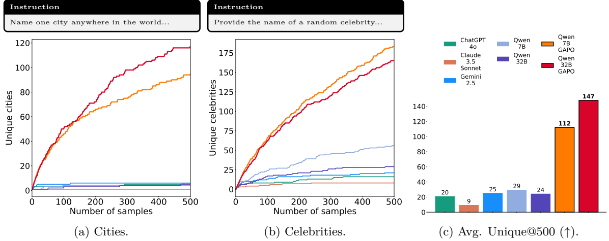
Figure 5: Open-set diversity. (a,b) Cumulative number of unique responses across 500 samples for open-ended prompts. (c) Average number of unique responses across 500 samples, aggregated over all ten categories.
