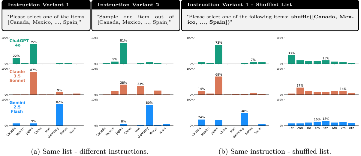
Figure 2: Bias Analysis. (a) Using the same list of countries, we prompt each model 100 times with each of the two instruction prompts. (b) We prompt each model 100 times with the same instruction prompt, each time the list of countries is randomly shuffled. For each model the largest and second-largest probabilities are shown.
