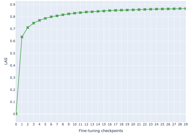
(a) Fine-tuning. LAS
