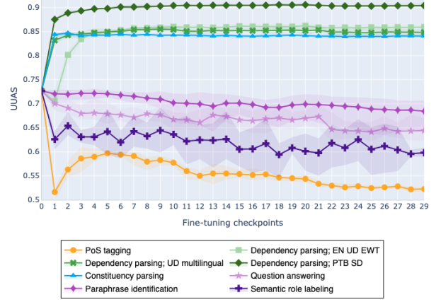
Figure 1: Tree distance evaluation. UAS evolution.
