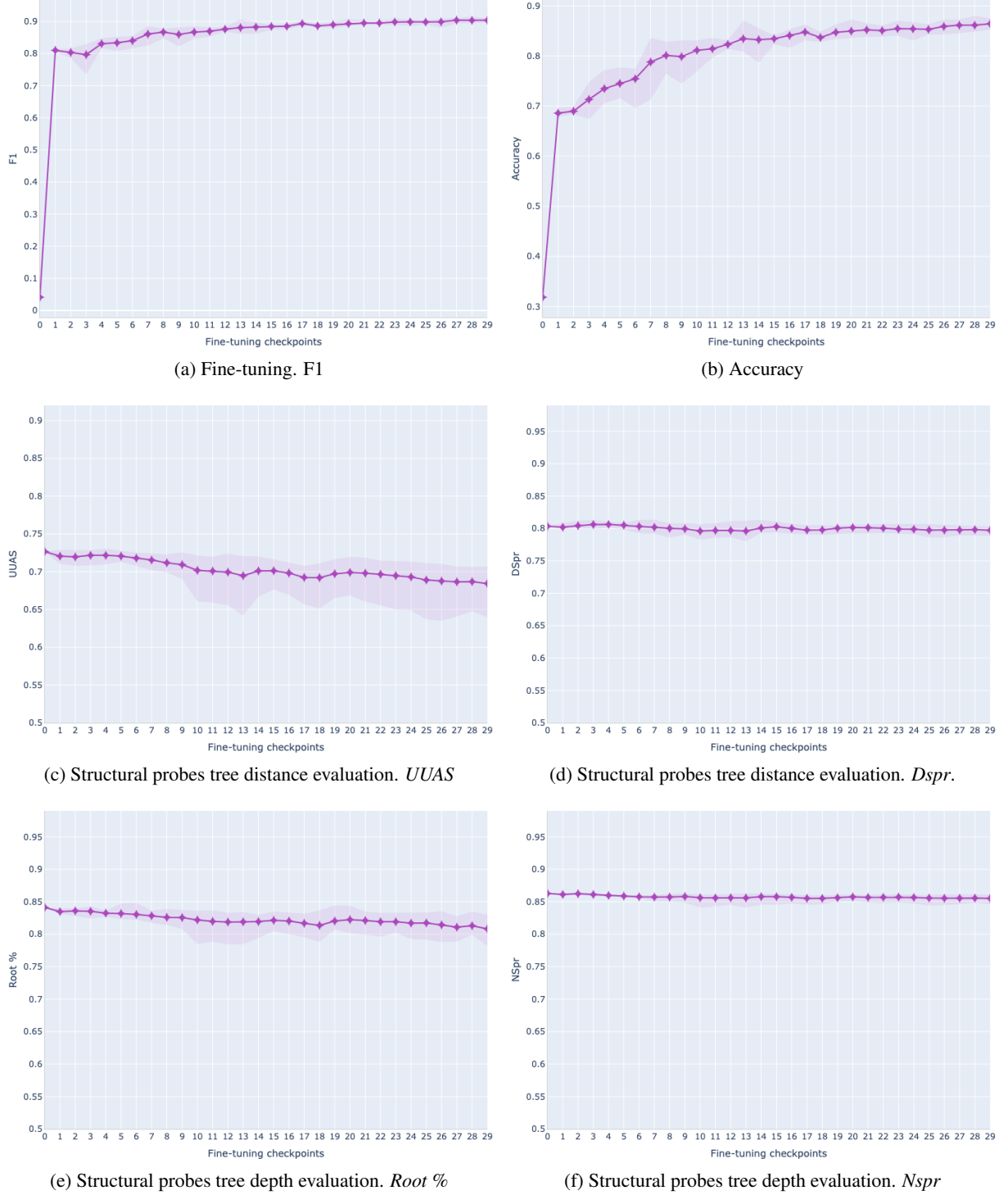
Figure 11: Paraphrase identification. Fine-tuning & probing metrics evolution.
