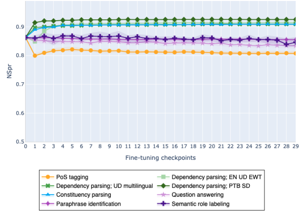
Figure 4: Tree depth evaluation. NSpr evolution.
