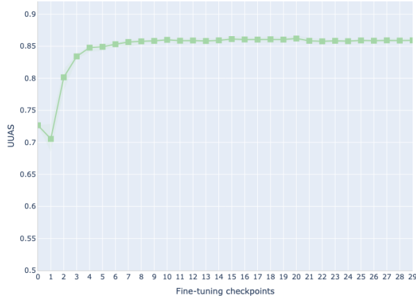
(b) Structural probes tree distance evaluation. UAS
