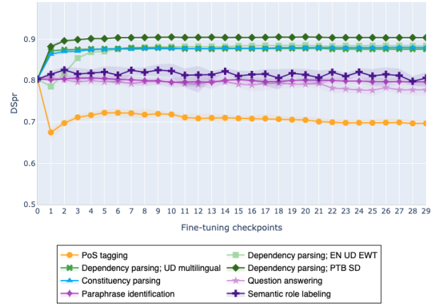
Figure 2: Tree distance evaluation. DSpr evolution.
